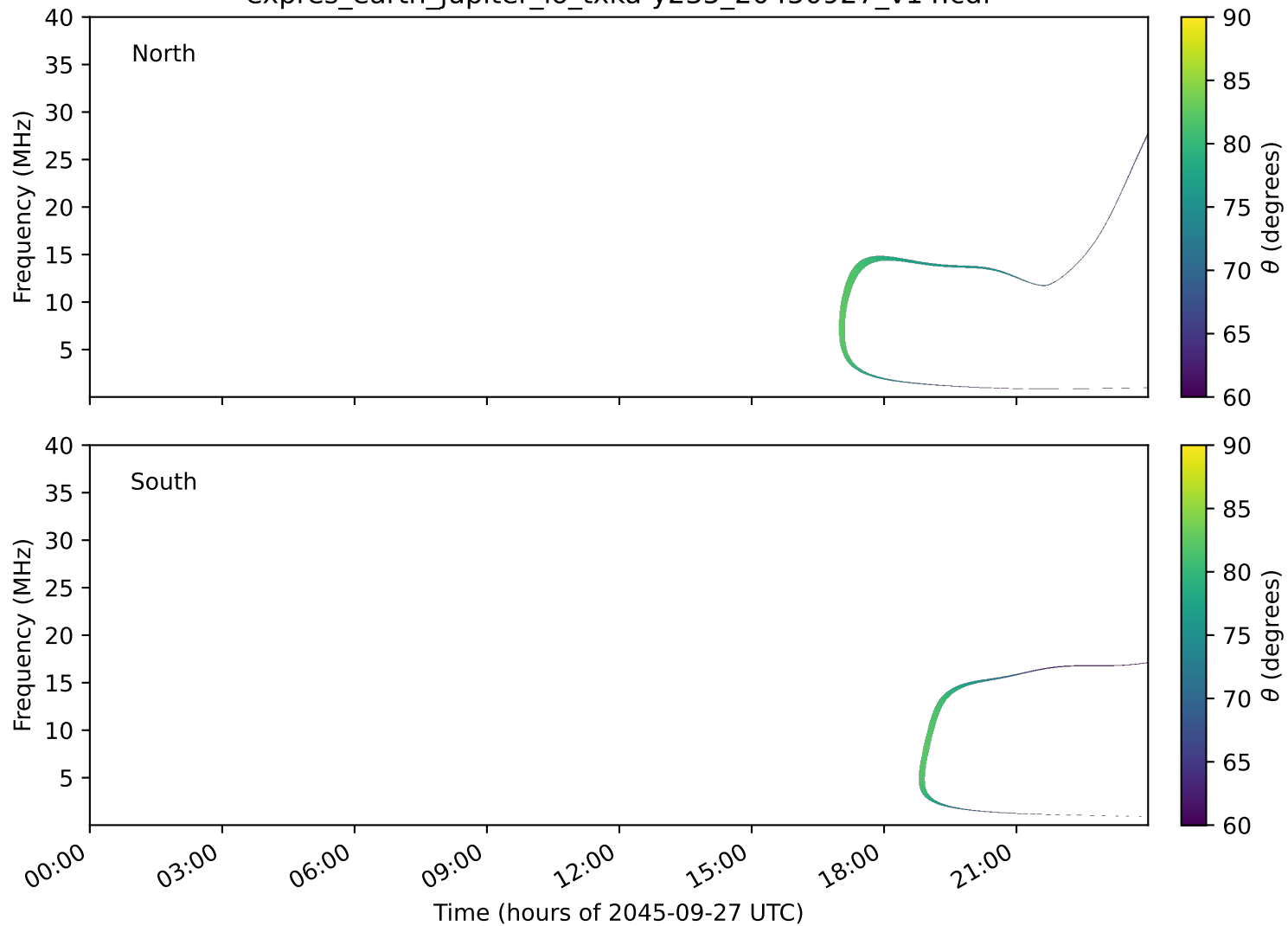
expres_earth_jupiter_io_txka-y235_20450927_v14.cdf
