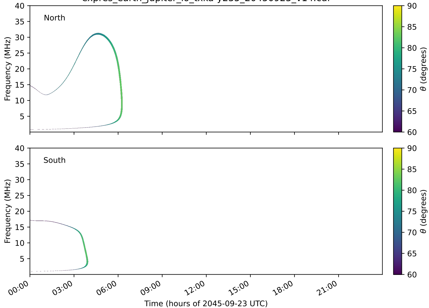
expres_earth_jupiter_io_txka-y235_20450923_v14.cdf
