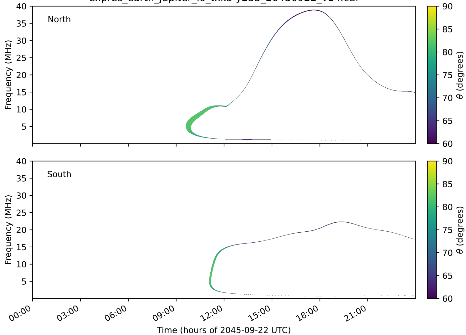
expres_earth_jupiter_io_txka-y235_20450922_v14.cdf
