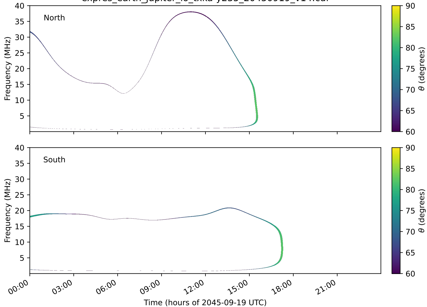
expres_earth_jupiter_io_txka-y235_20450919_v14.cdf
