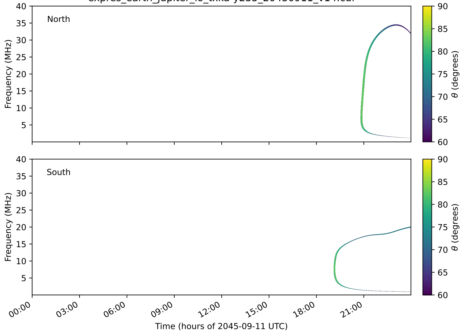
expres_earth_jupiter_io_txka-y235_20450911_v14.cdf
