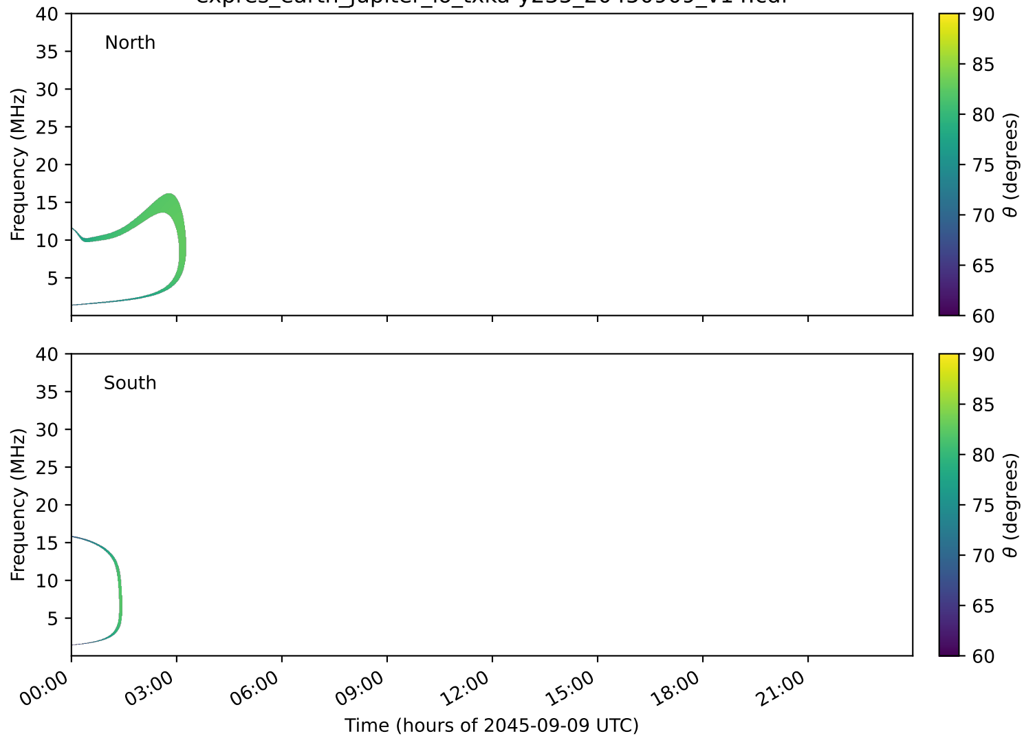
expres_earth_jupiter_io_txka-y235_20450909_v14.cdf
