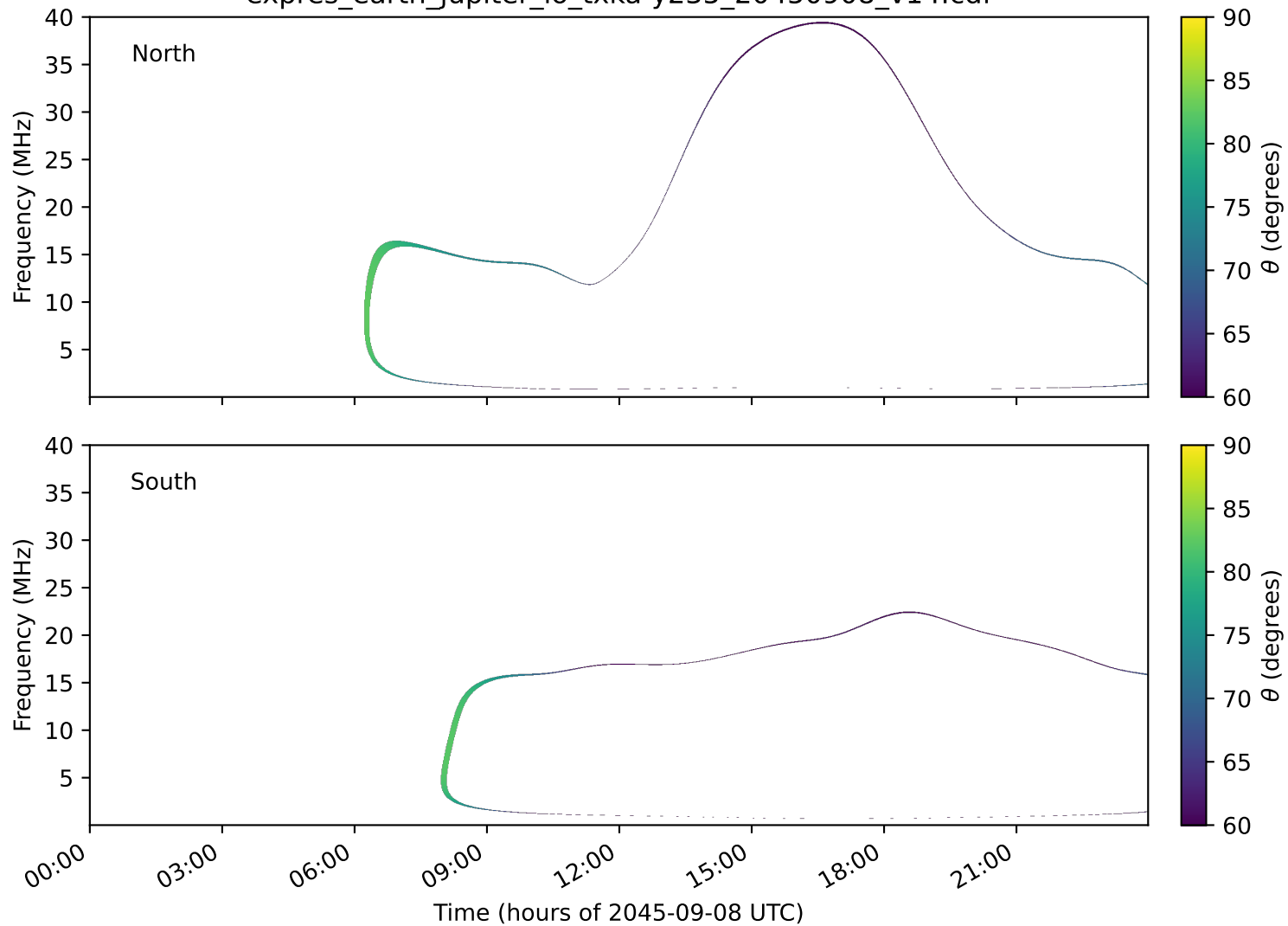
expres_earth_jupiter_io_txka-y235_20450908_v14.cdf
