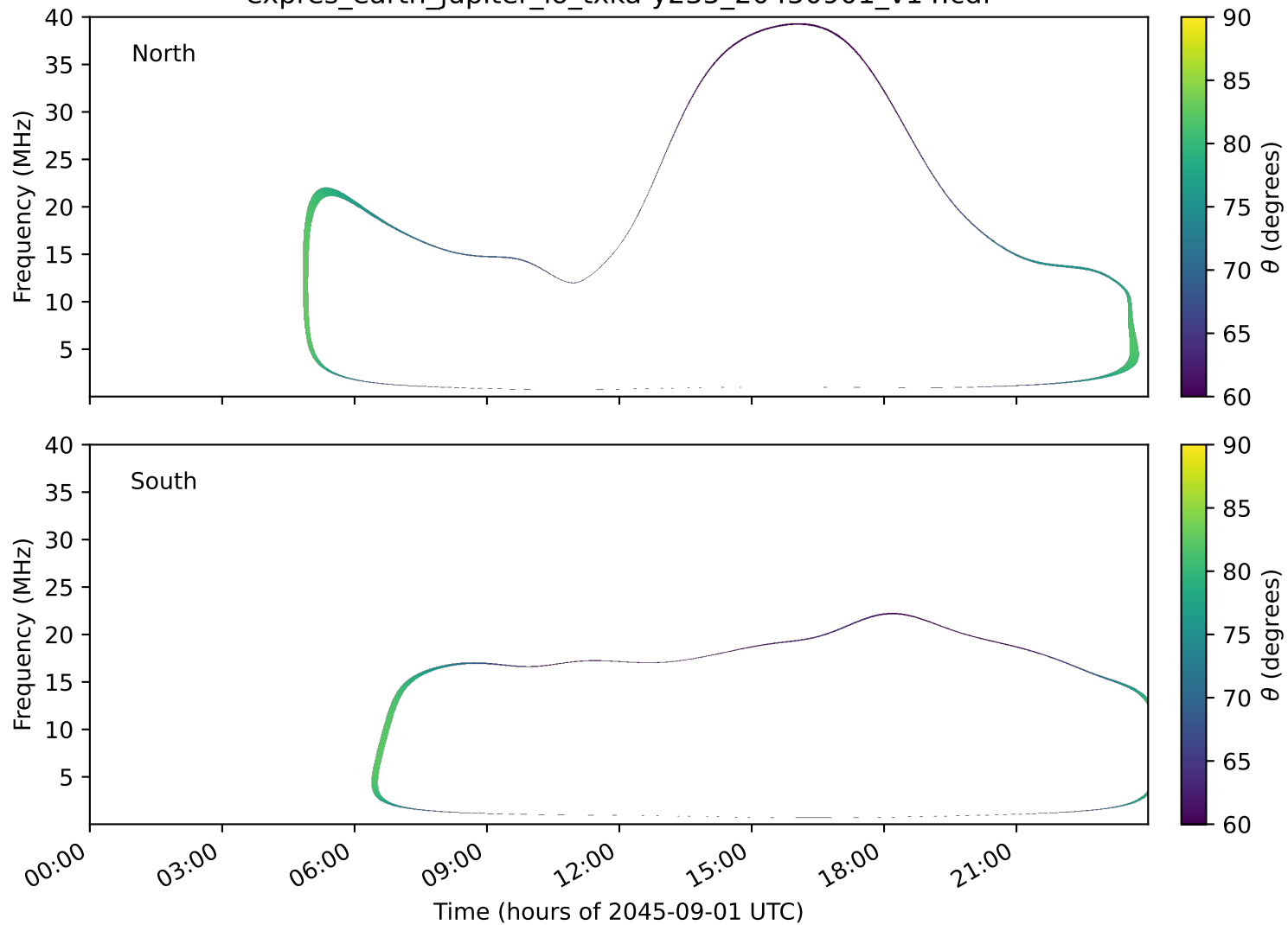
expres_earth_jupiter_io_txka-y235_20450901_v14.cdf
