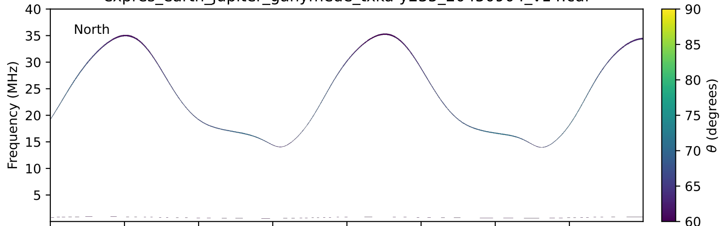
expres_earth_jupiter_ganymede_txka-y235_20450904_v14.cdf
