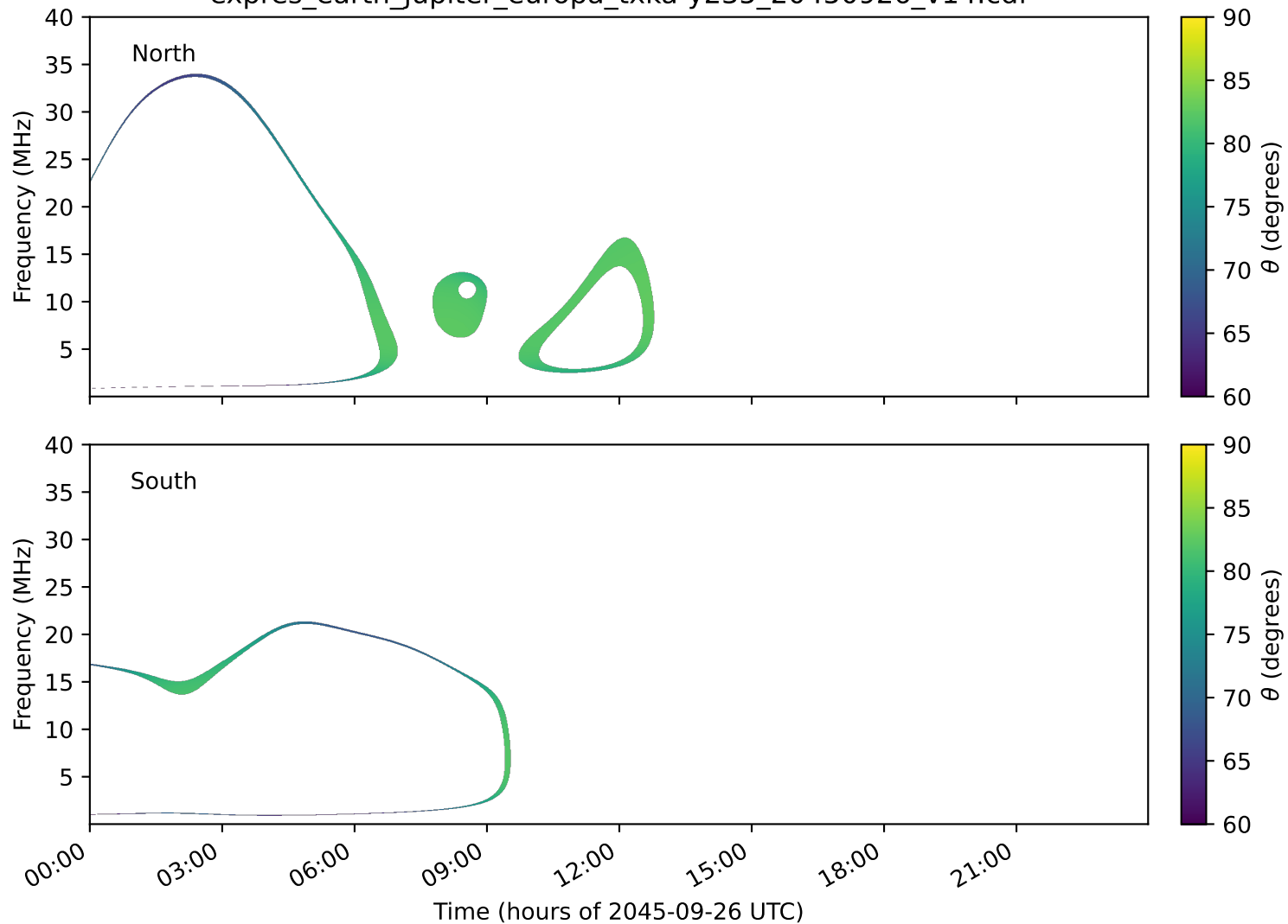
expres_earth_jupiter_europa_txka-y235_20450926_v14.cdf
