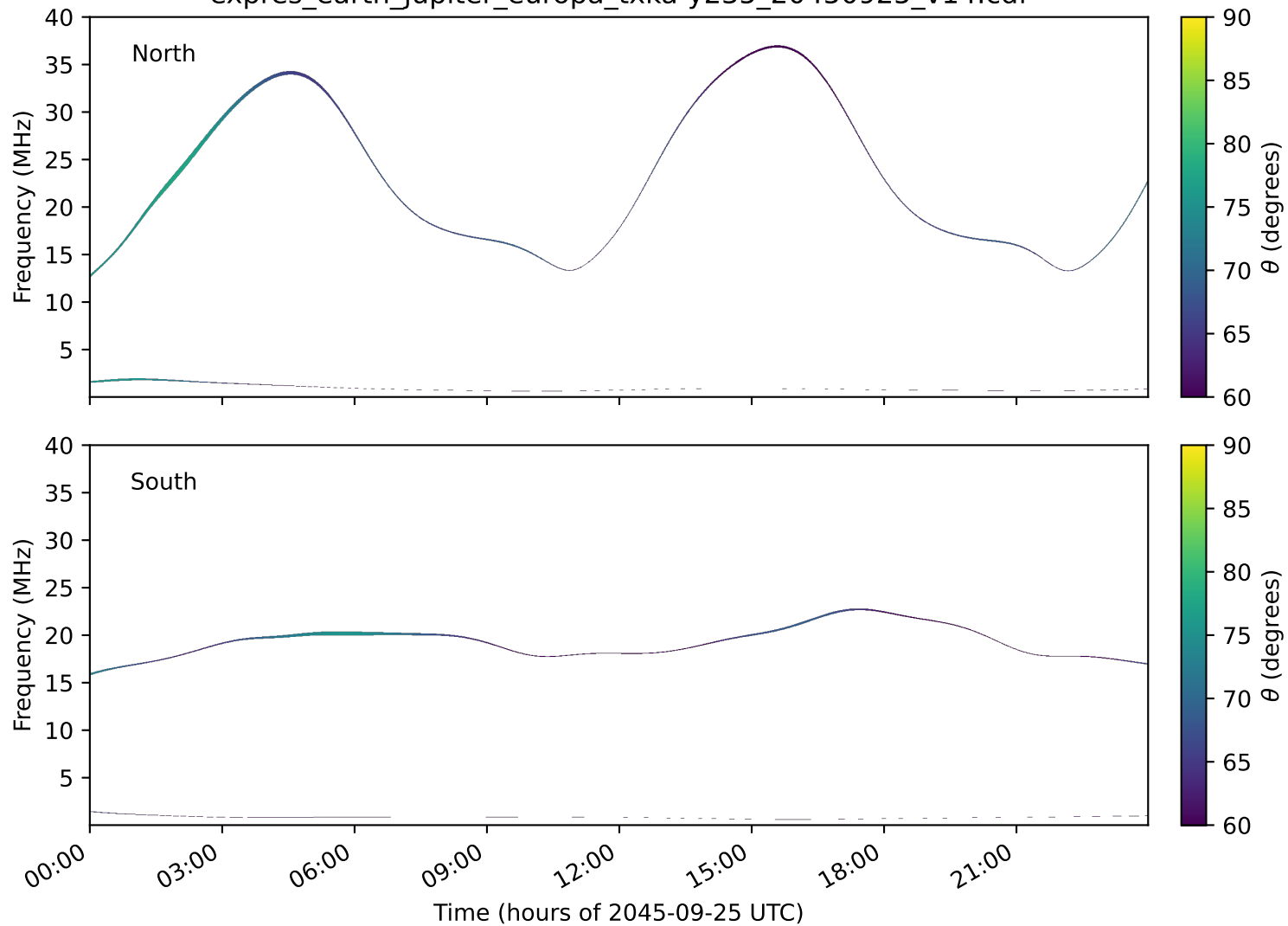
expres_earth_jupiter_europa_txka-y235_20450925_v14.cdf
