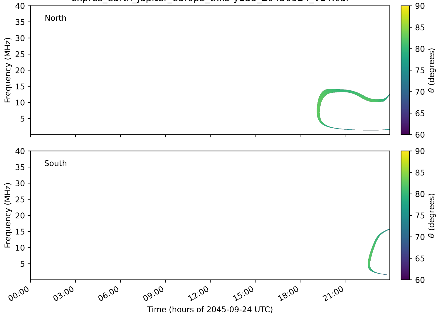
expres_earth_jupiter_europa_txka-y235_20450924_v14.cdf
