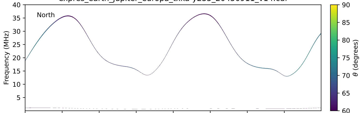
expres_earth_jupiter_europa_txka-y235_20450911_v14.cdf
