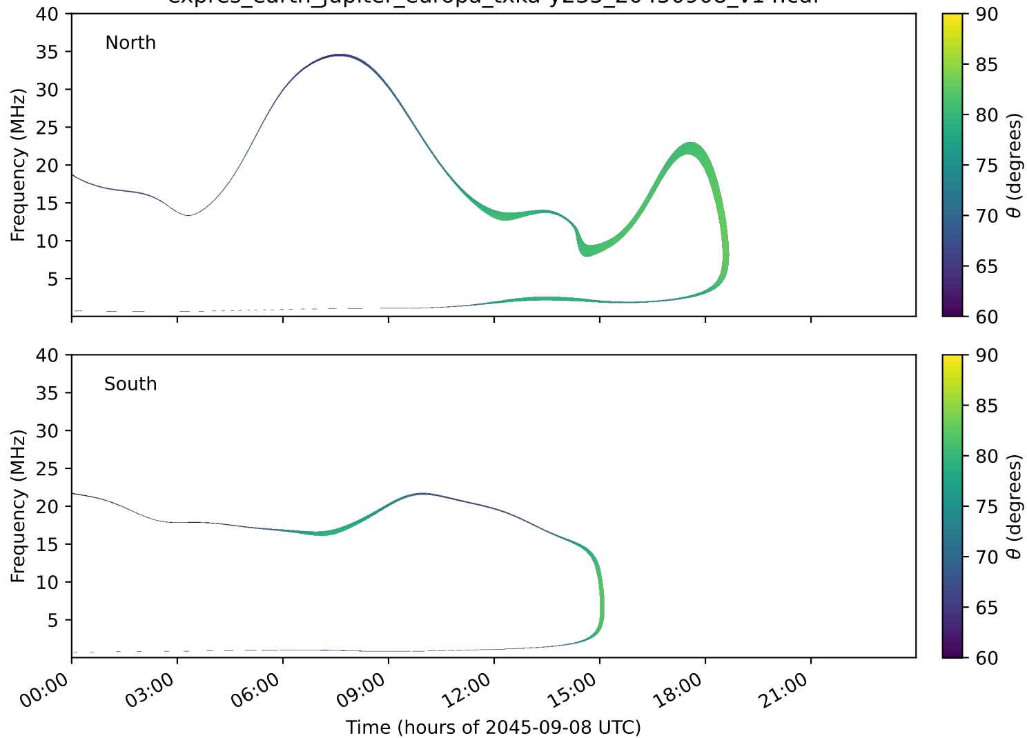
expres_earth_jupiter_europa_txka-y235_20450908_v14.cdf
