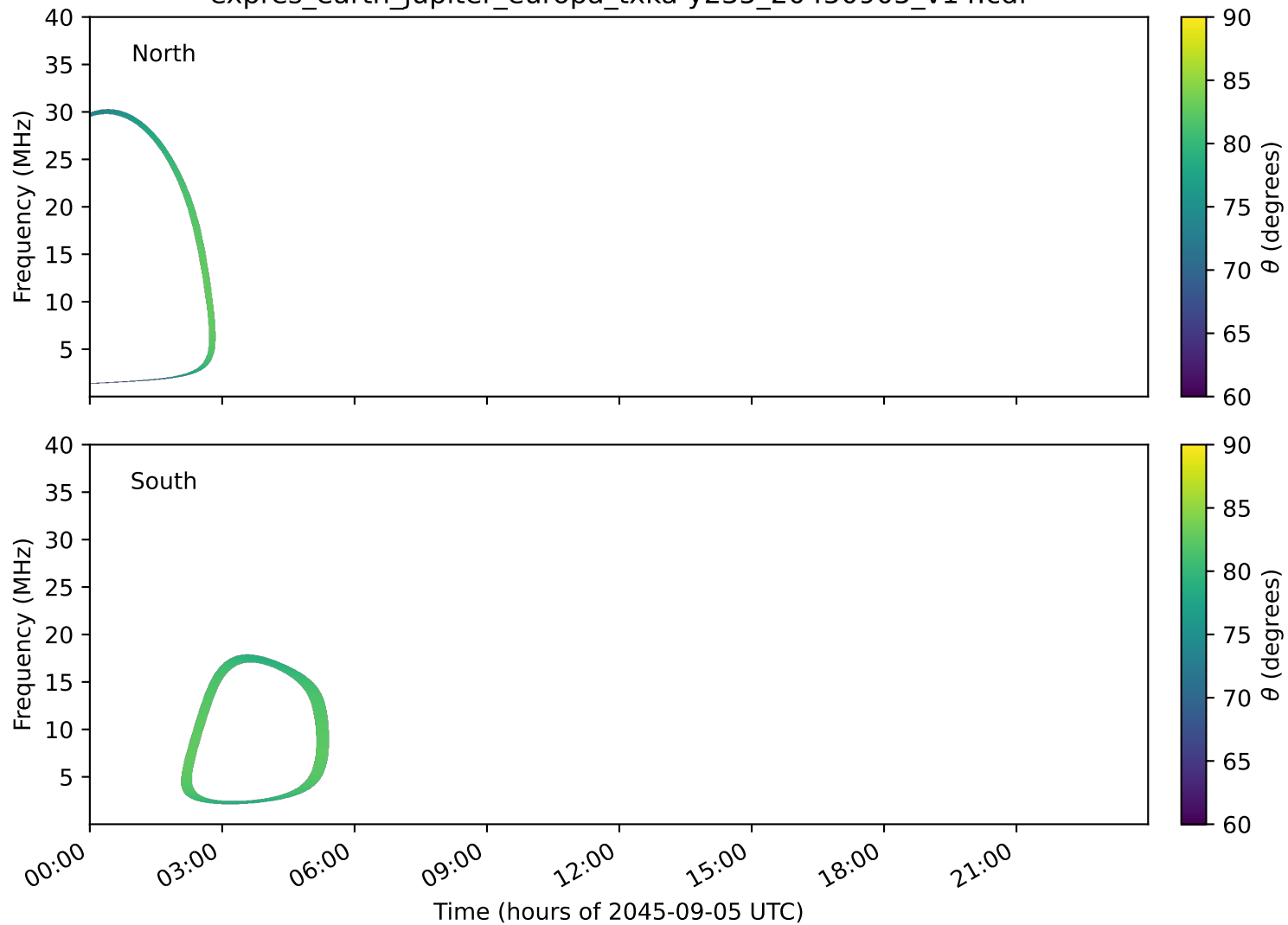
expres_earth_jupiter_europa_txka-y235_20450905_v14.cdf
