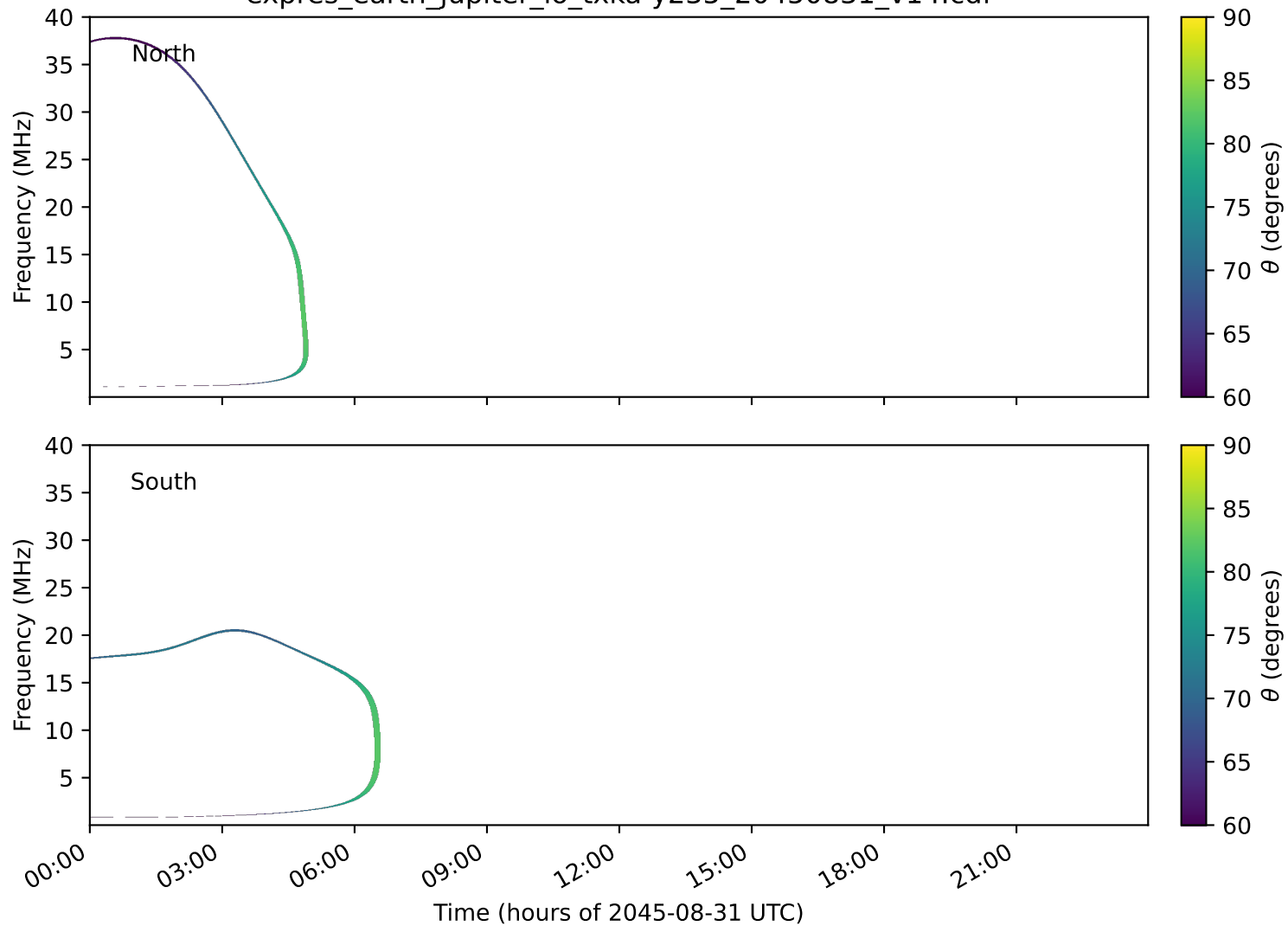
expres_earth_jupiter_io_txka-y235_20450831_v14.cdf
