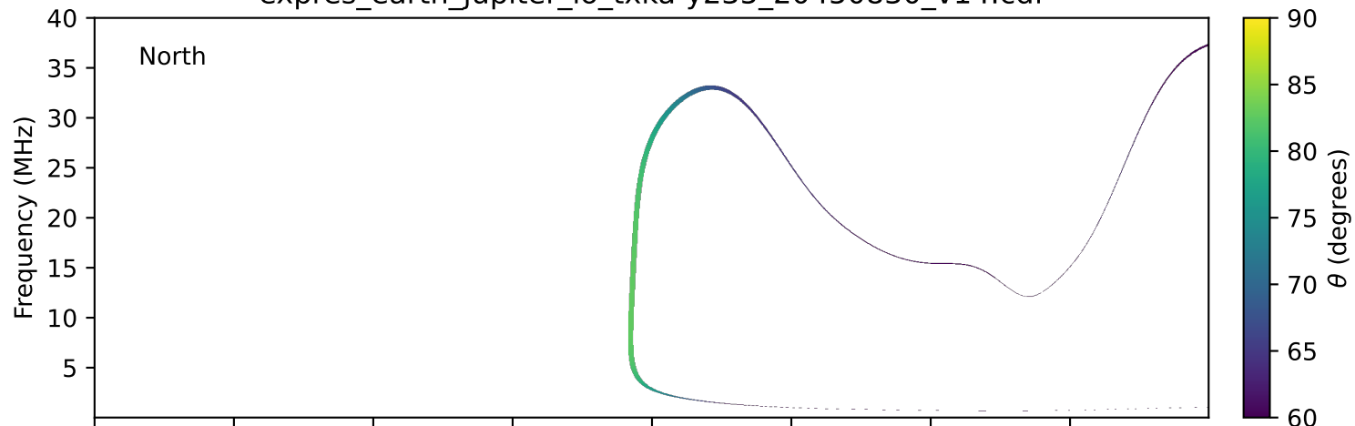
expres_earth_jupiter_io_txka-y235_20450830_v14.cdf
