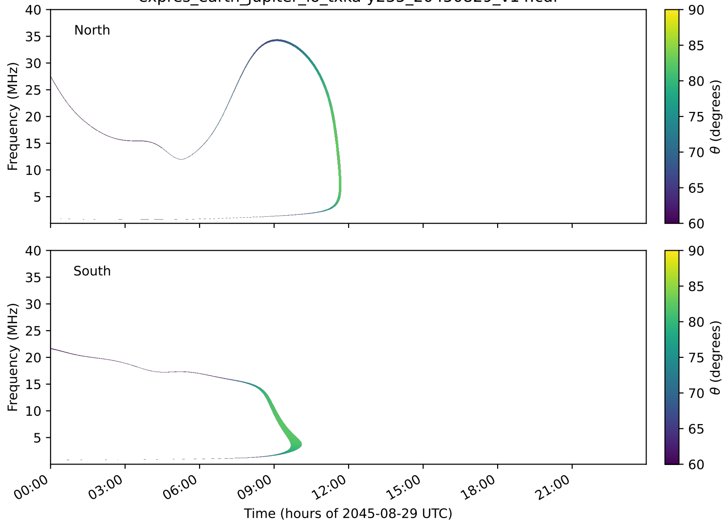
expres_earth_jupiter_io_txka-y235_20450829_v14.cdf
