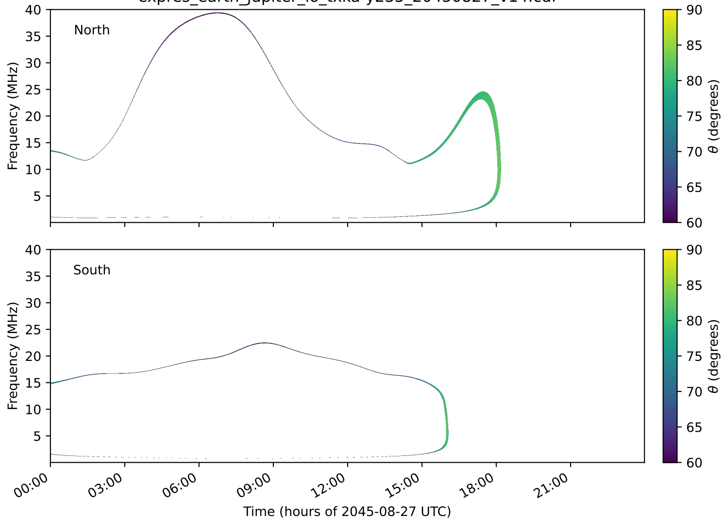
expres_earth_jupiter_io_txka-y235_20450827_v14.cdf
