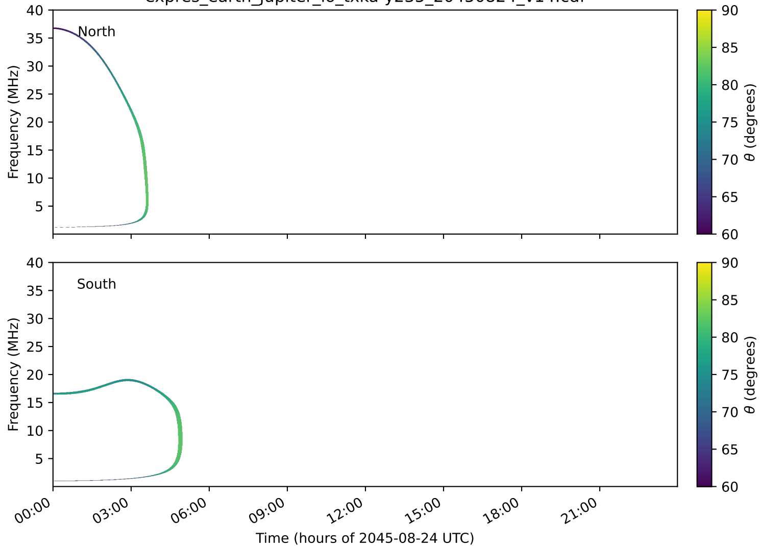
expres_earth_jupiter_io_txka-y235_20450824_v14.cdf
