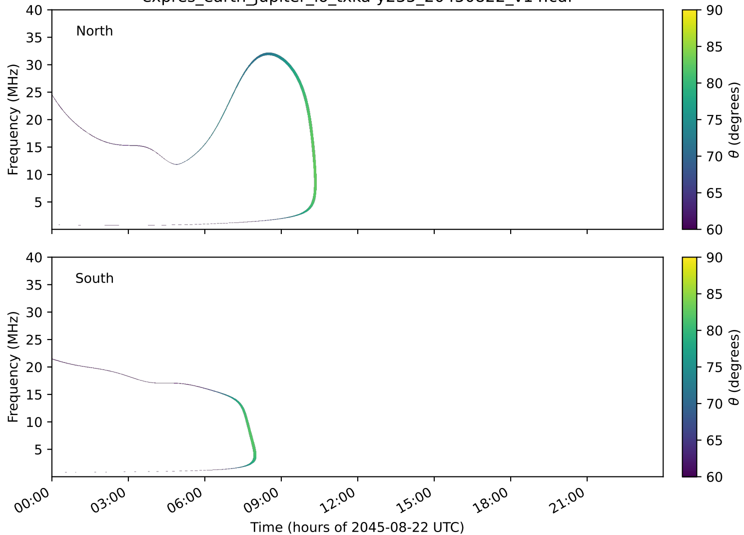
expres_earth_jupiter_io_txka-y235_20450822_v14.cdf
