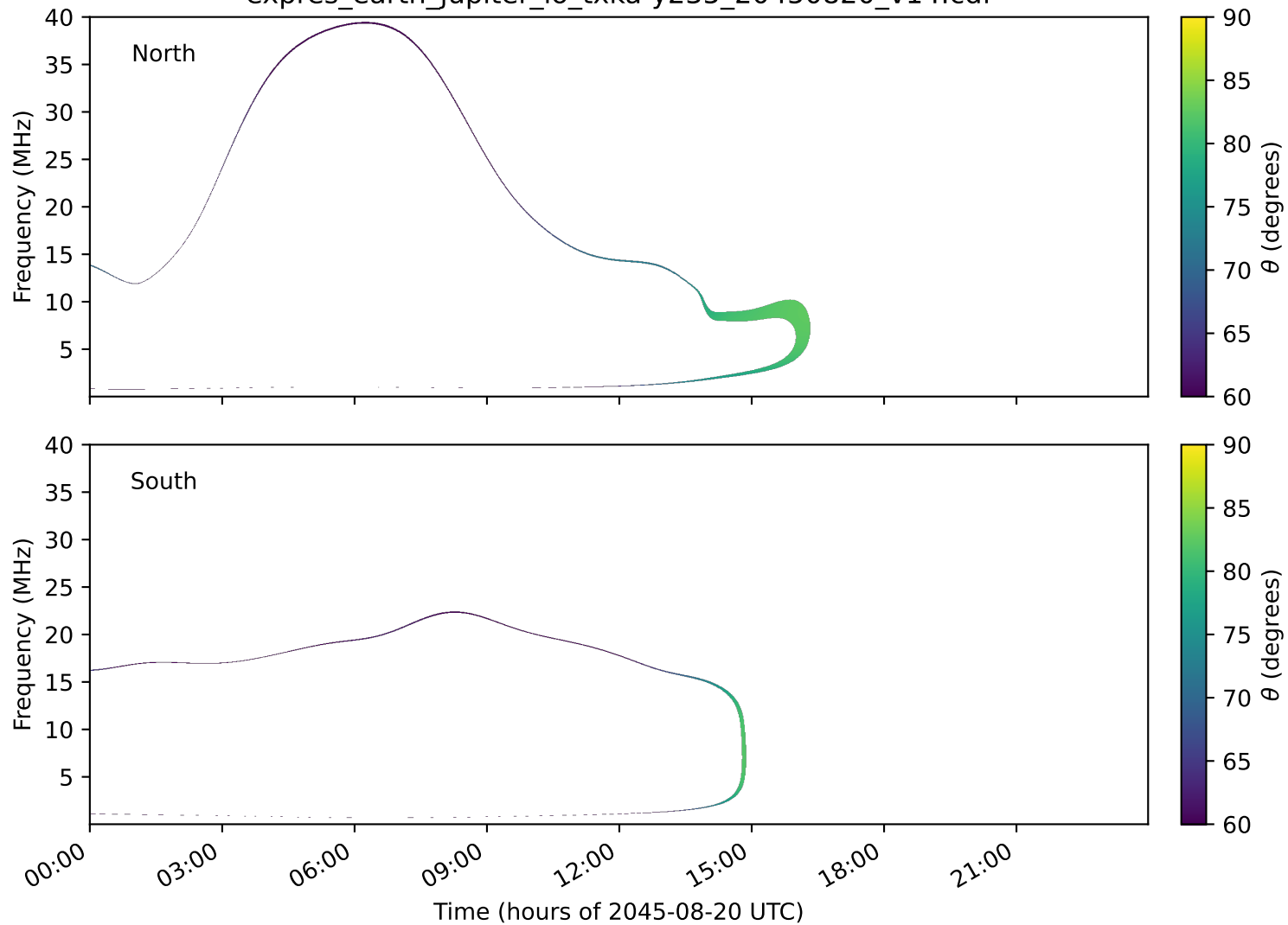
expres_earth_jupiter_io_txka-y235_20450820_v14.cdf
