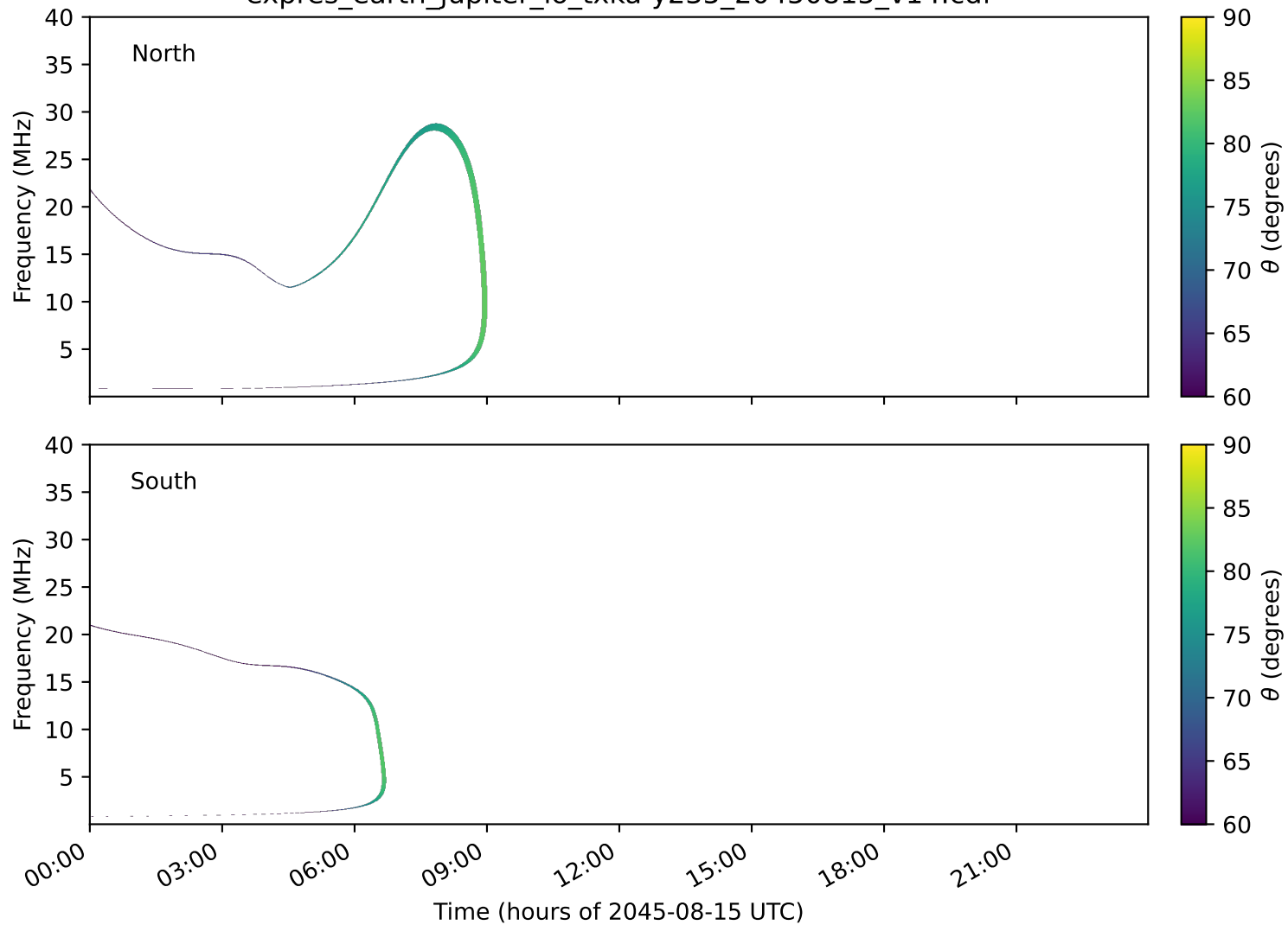
expres_earth_jupiter_io_txka-y235_20450815_v14.cdf
