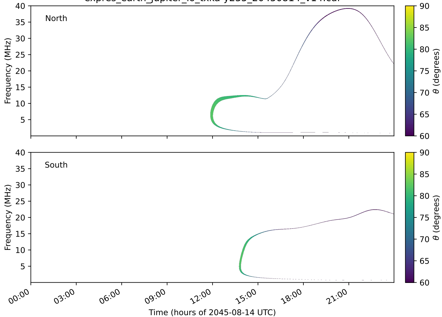
expres_earth_jupiter_io_txka-y235_20450814_v14.cdf
