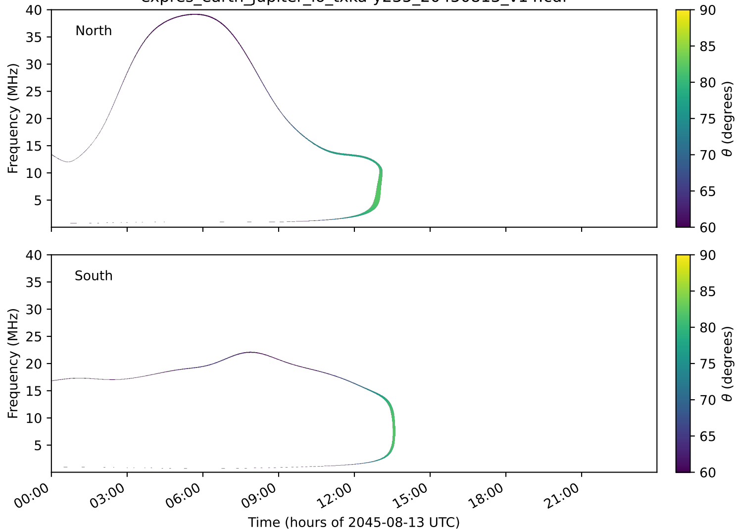
expres_earth_jupiter_io_txka-y235_20450813_v14.cdf
