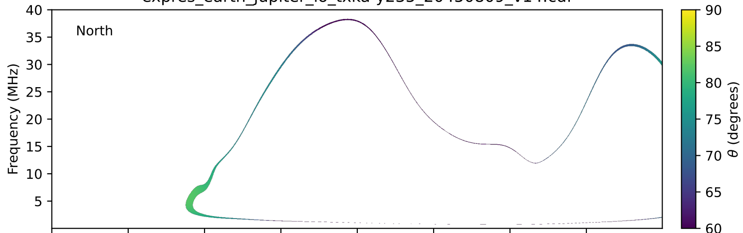
expres_earth_jupiter_io_txka-y235_20450809_v14.cdf
