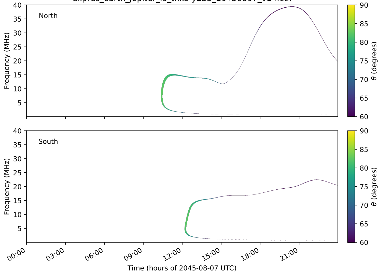
expres_earth_jupiter_io_txka-y235_20450807_v14.cdf
