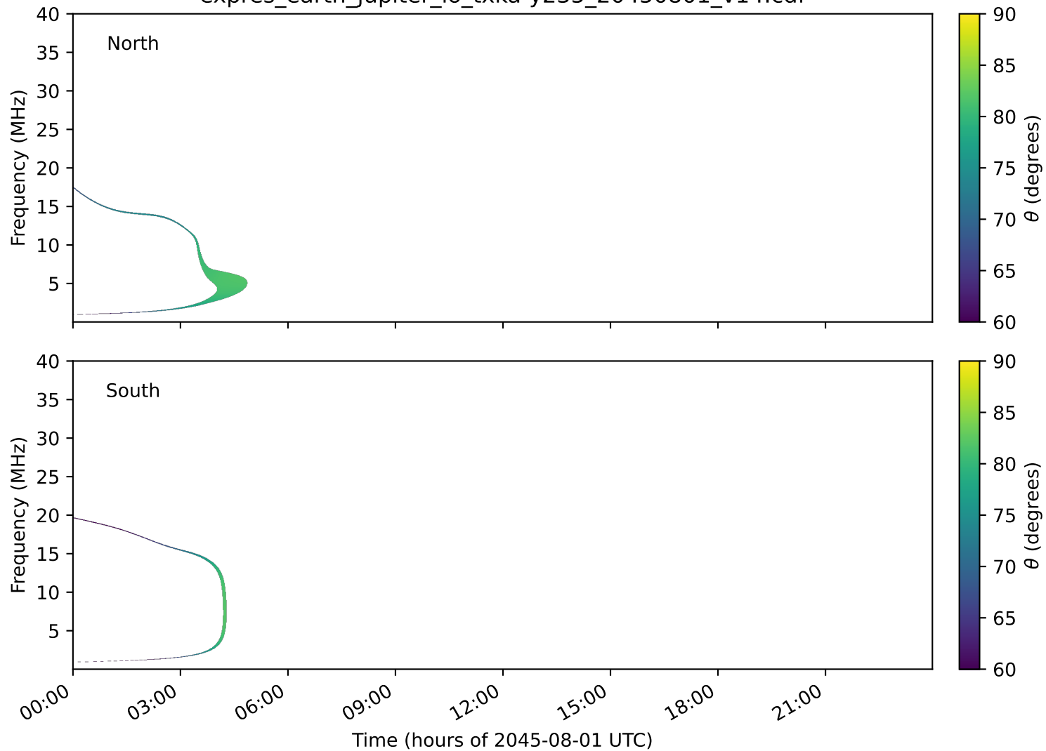
expres_earth_jupiter_io_txka-y235_20450801_v14.cdf
