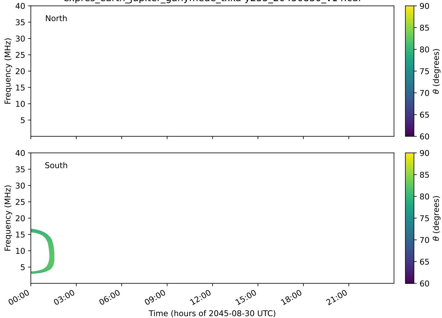
expres_earth_jupiter_ganymede_txka-y235_20450830_v14.cdf
