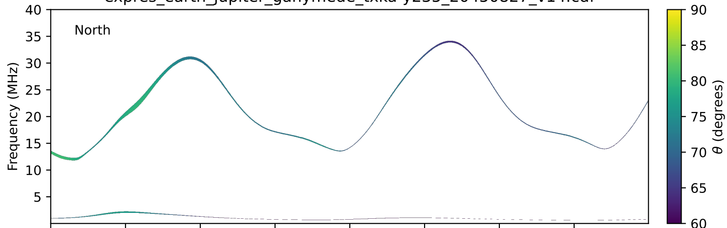
expres_earth_jupiter_ganymede_txka-y235_20450827_v14.cdf
