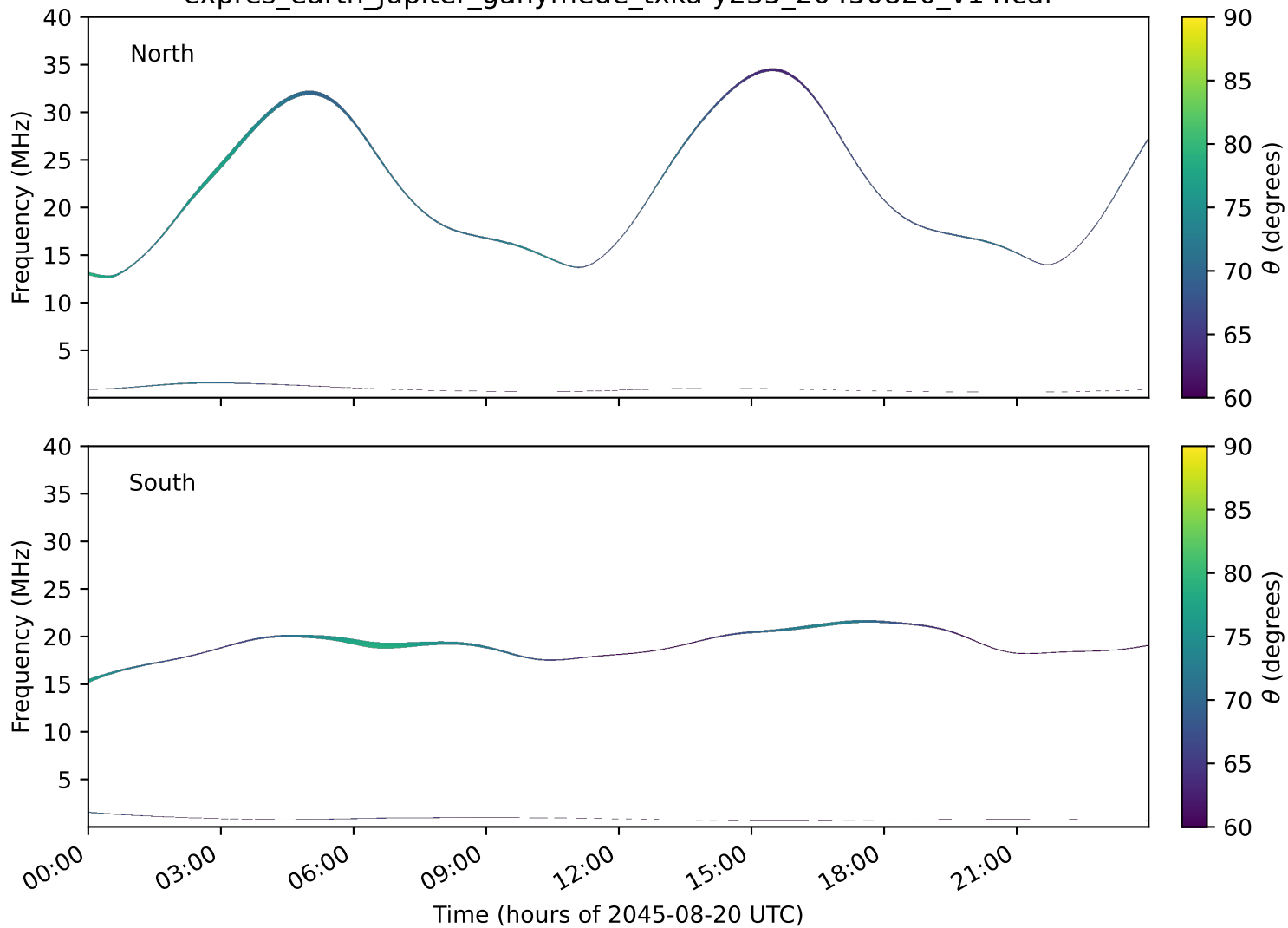
expres_earth_jupiter_ganymede_txka-y235_20450820_v14.cdf
