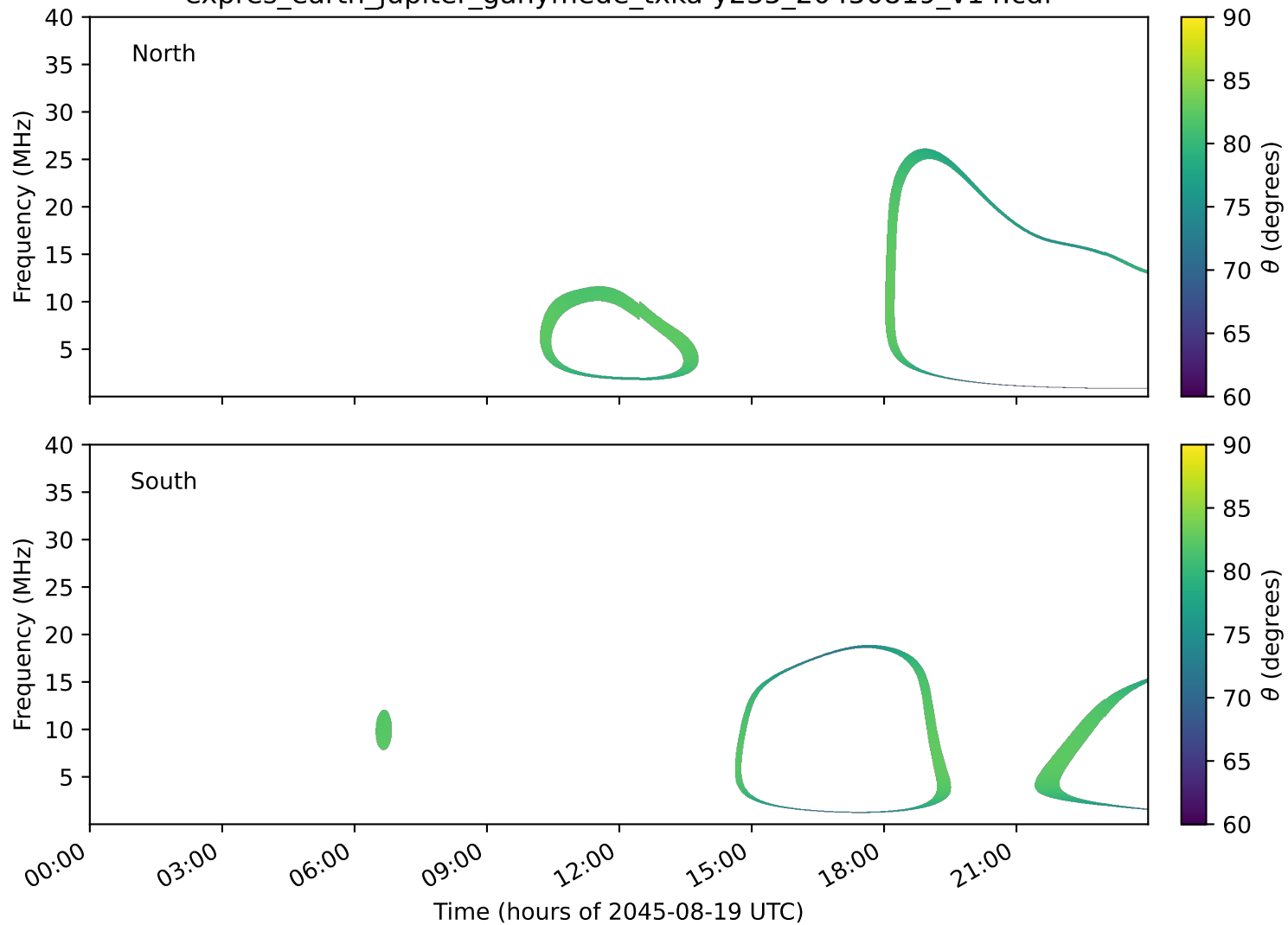
expres_earth_jupiter_ganymede_txka-y235_20450819_v14.cdf
