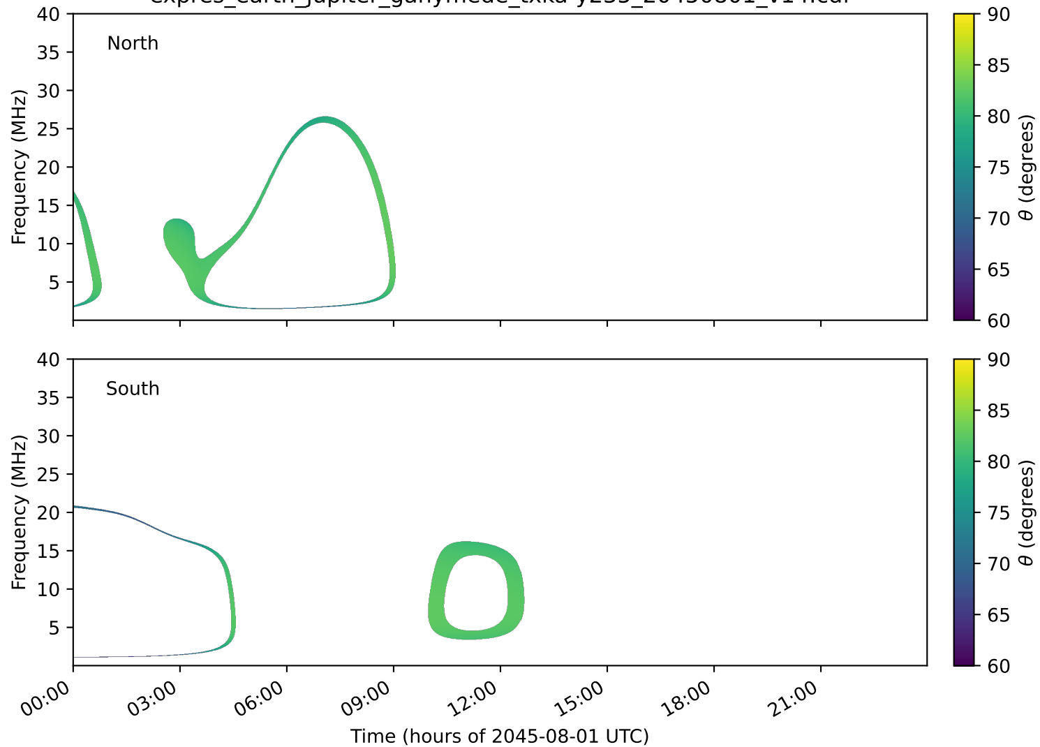
expres_earth_jupiter_ganymede_txka-y235_20450801_v14.cdf
