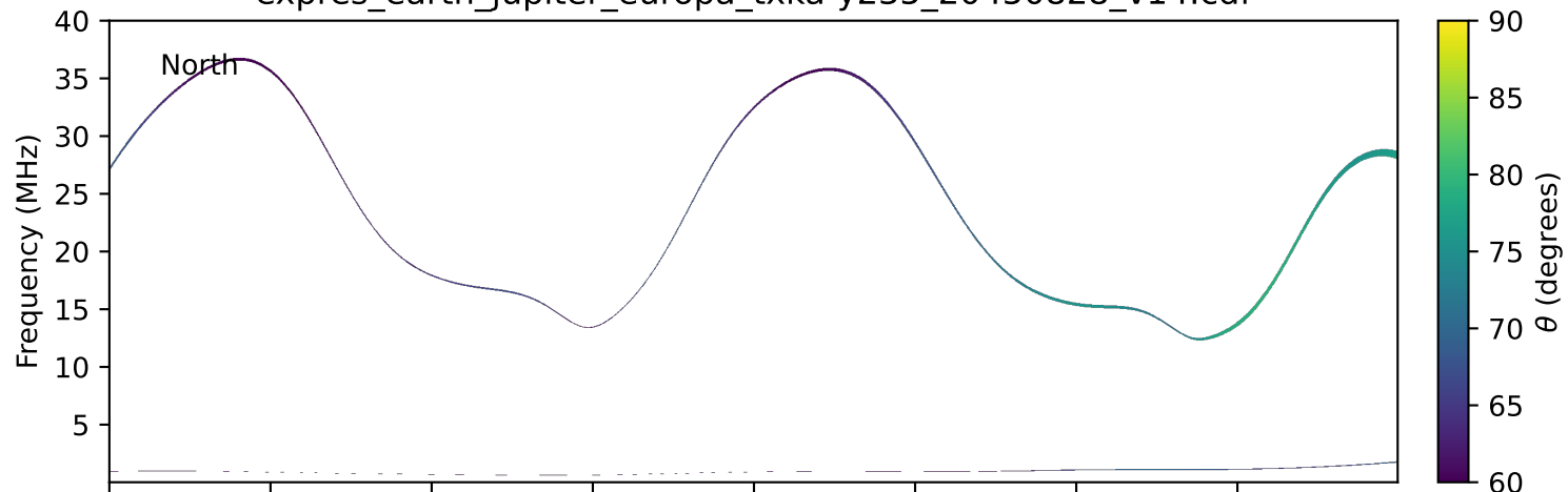
expres_earth_jupiter_europa_txka-y235_20450828_v14.cdf
