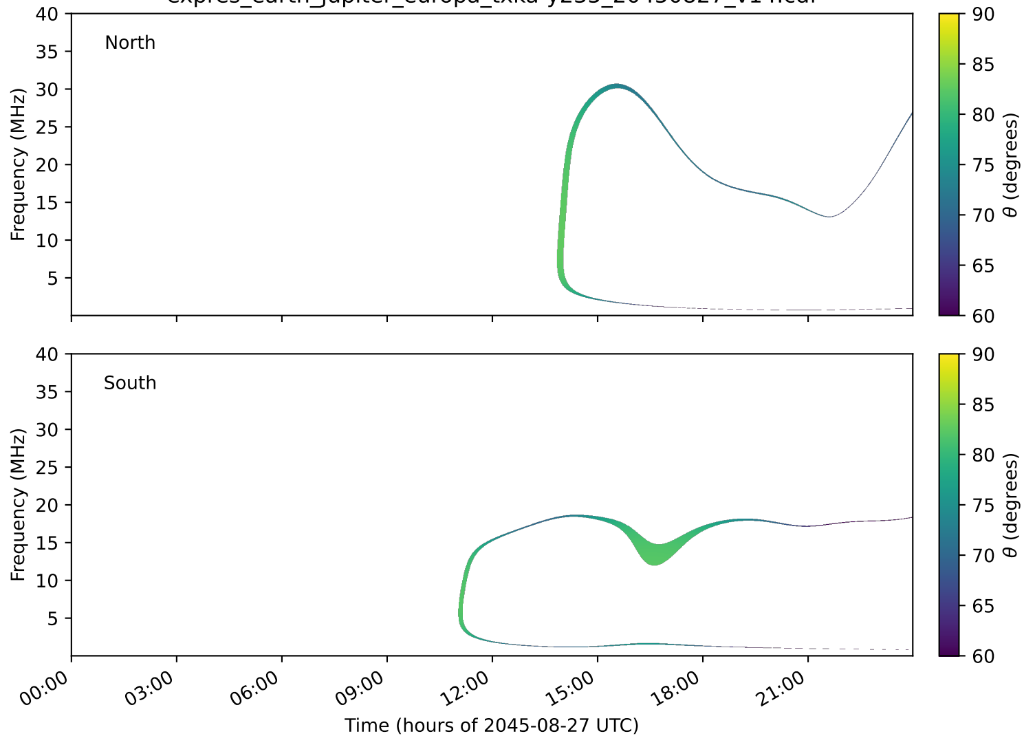
expres_earth_jupiter_europa_txka-y235_20450827_v14.cdf
