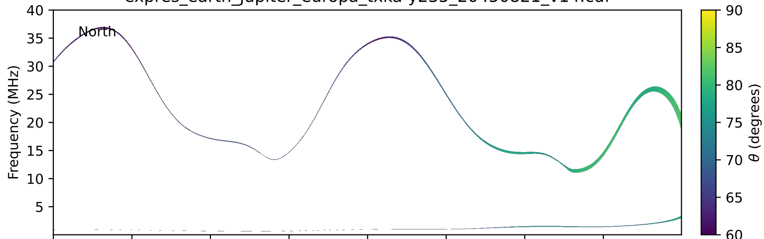
expres_earth_jupiter_europa_txka-y235_20450821_v14.cdf
