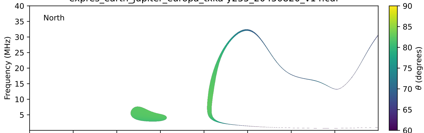
expres_earth_jupiter_europa_txka-y235_20450820_v14.cdf
