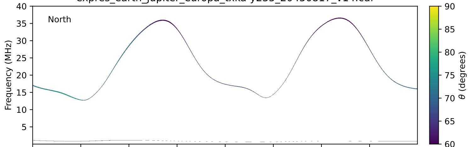
expres_earth_jupiter_europa_txka-y235_20450817_v14.cdf
