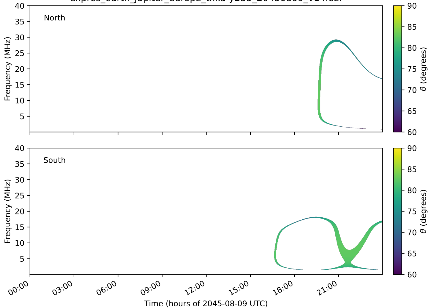
expres_earth_jupiter_europa_txka-y235_20450809_v14.cdf
