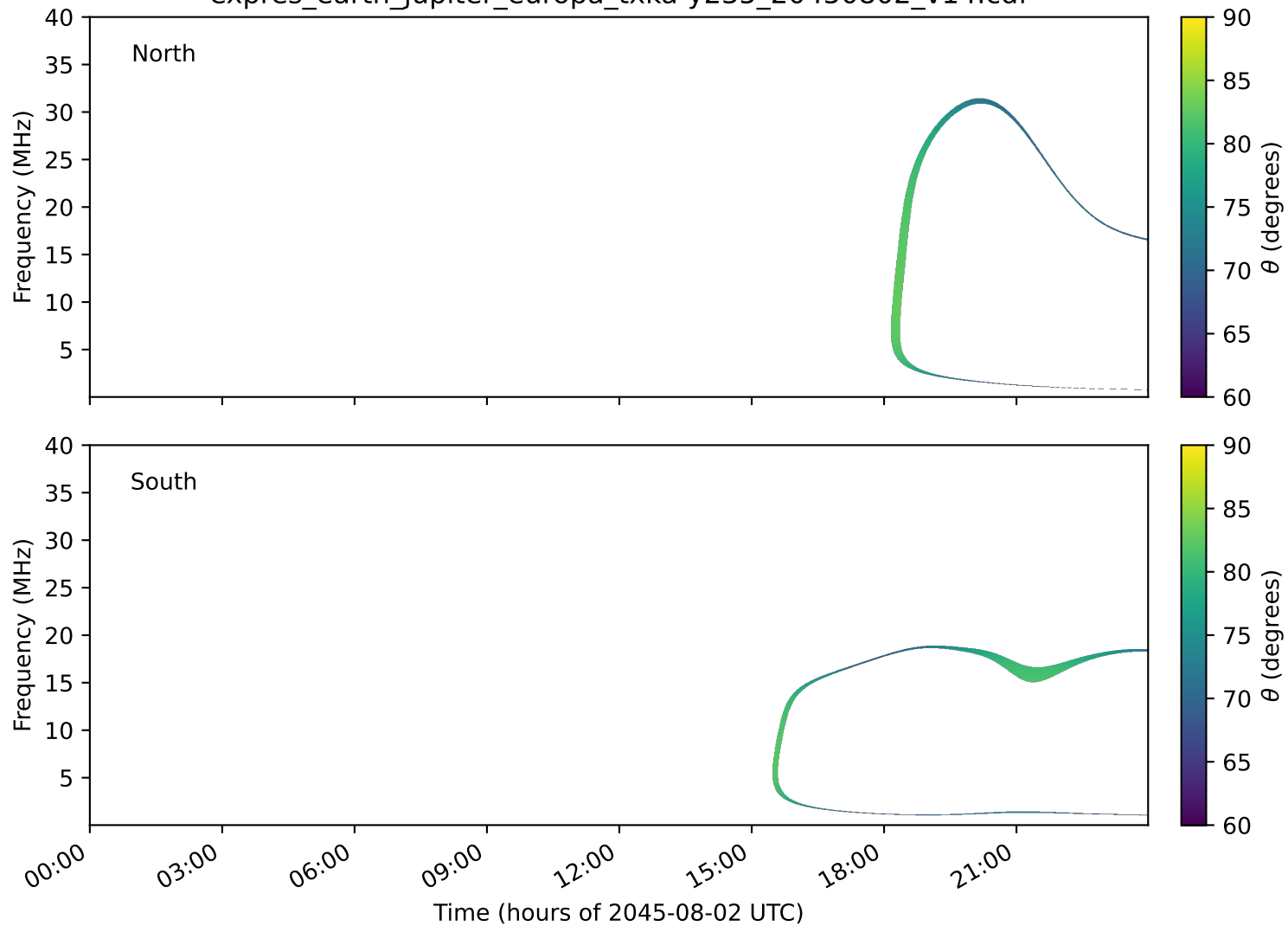
expres_earth_jupiter_europa_txka-y235_20450802_v14.cdf
