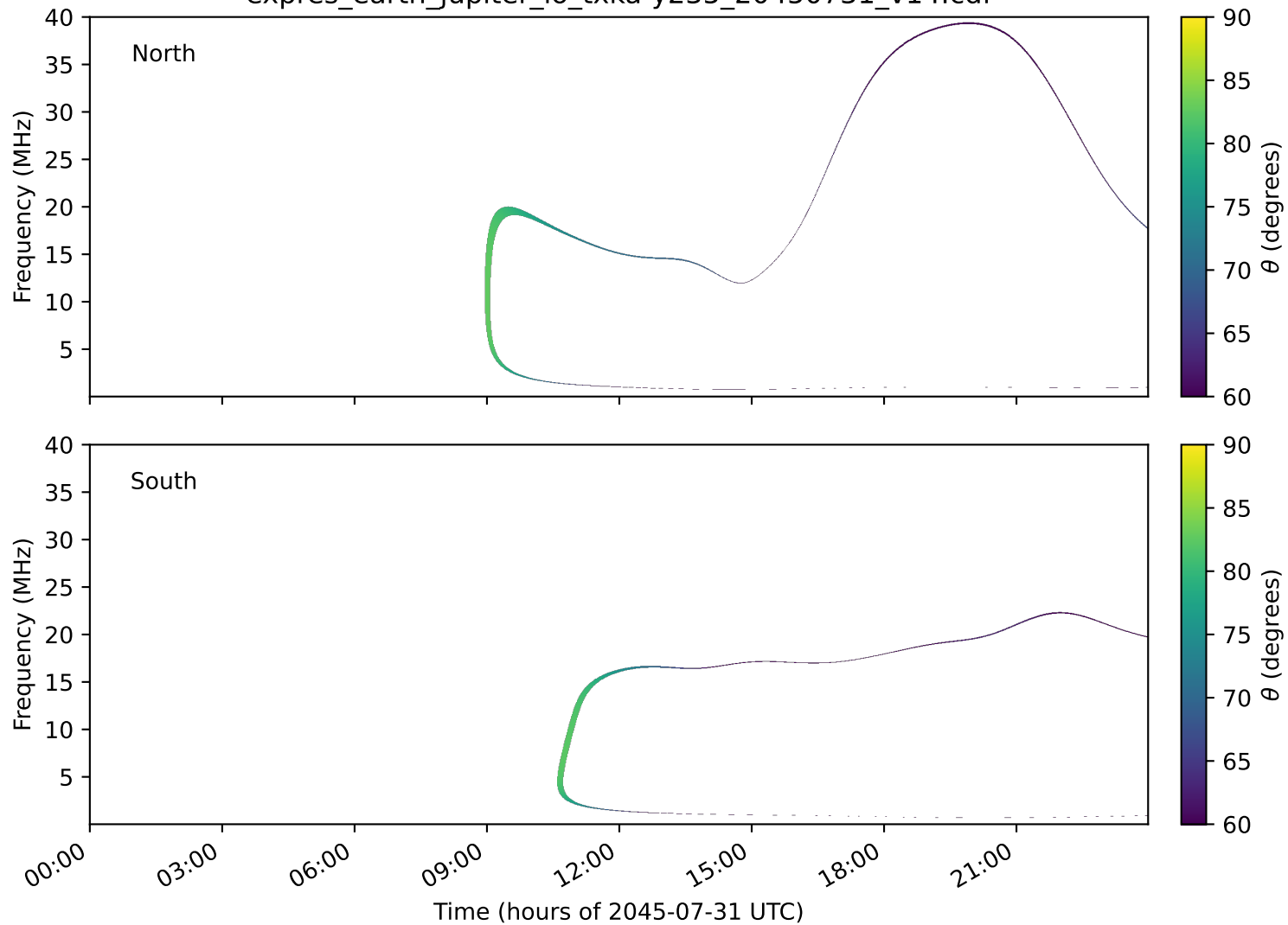
expres_earth_jupiter_io_txka-y235_20450731_v14.cdf
