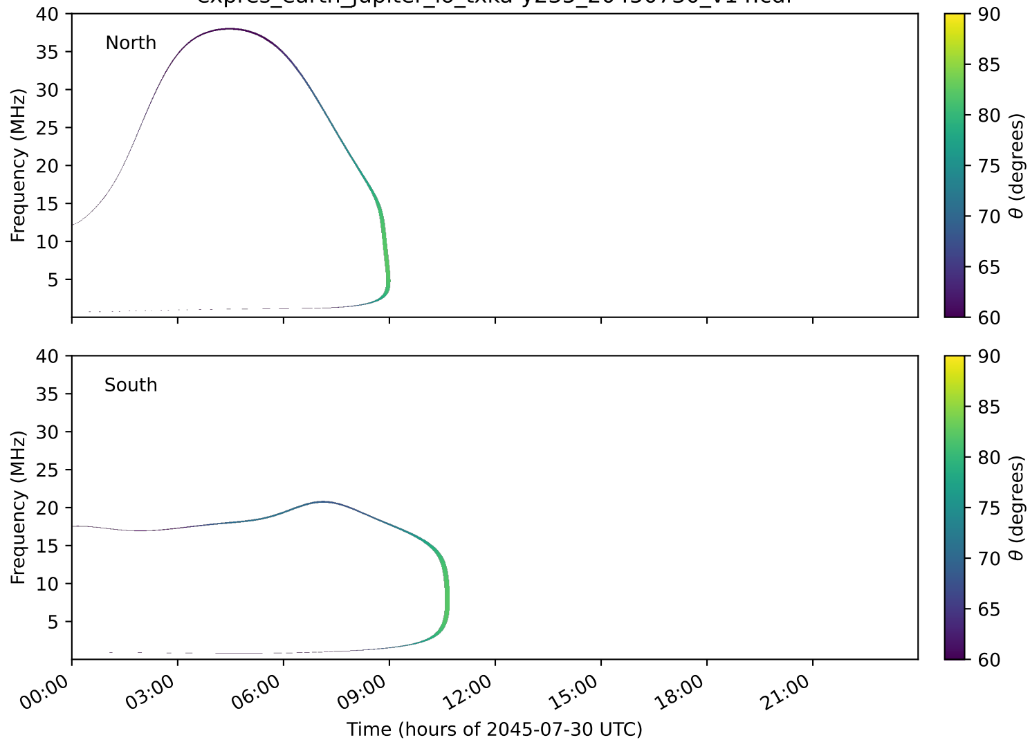
expres_earth_jupiter_io_txka-y235_20450730_v14.cdf
