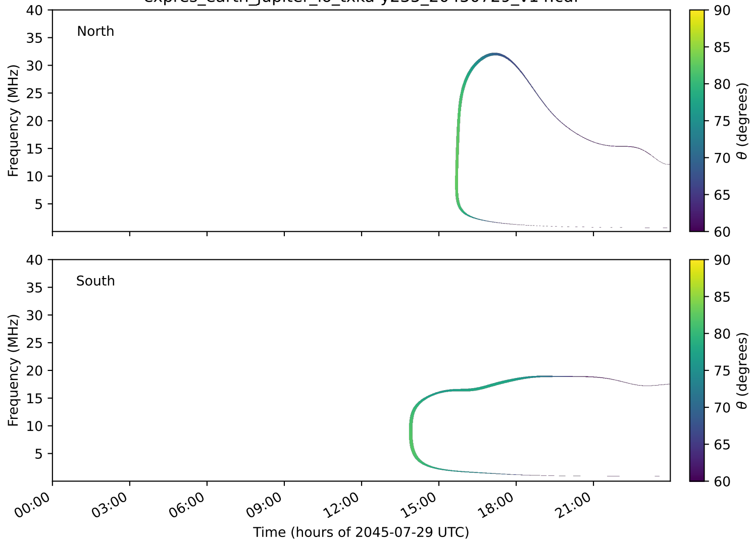
expres_earth_jupiter_io_txka-y235_20450729_v14.cdf
