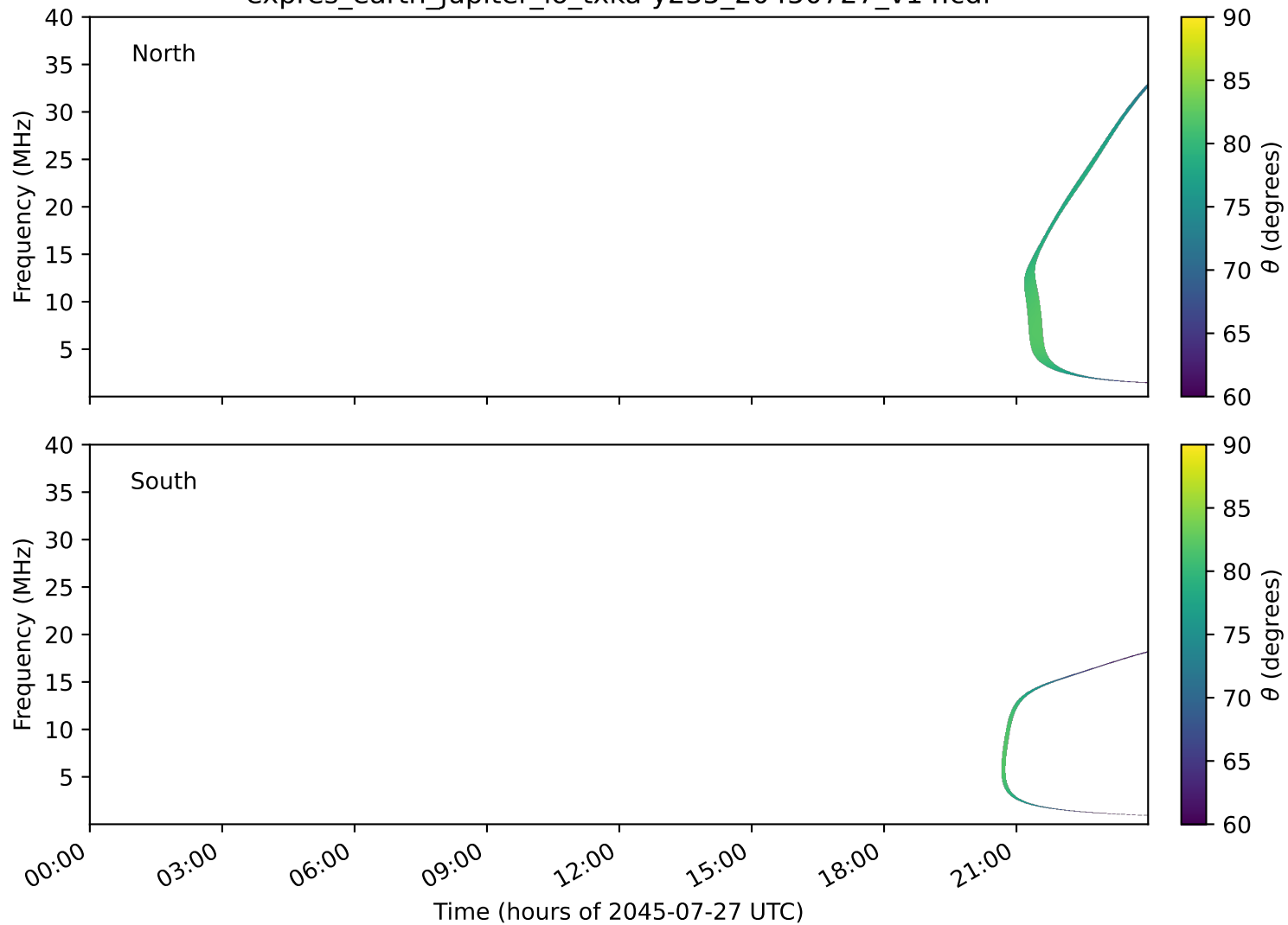
expres_earth_jupiter_io_txka-y235_20450727_v14.cdf
