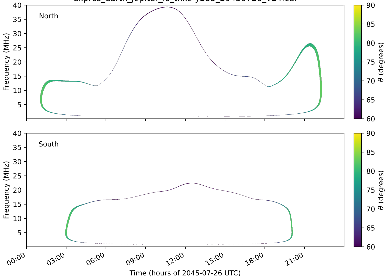
expres_earth_jupiter_io_txka-y235_20450726_v14.cdf
