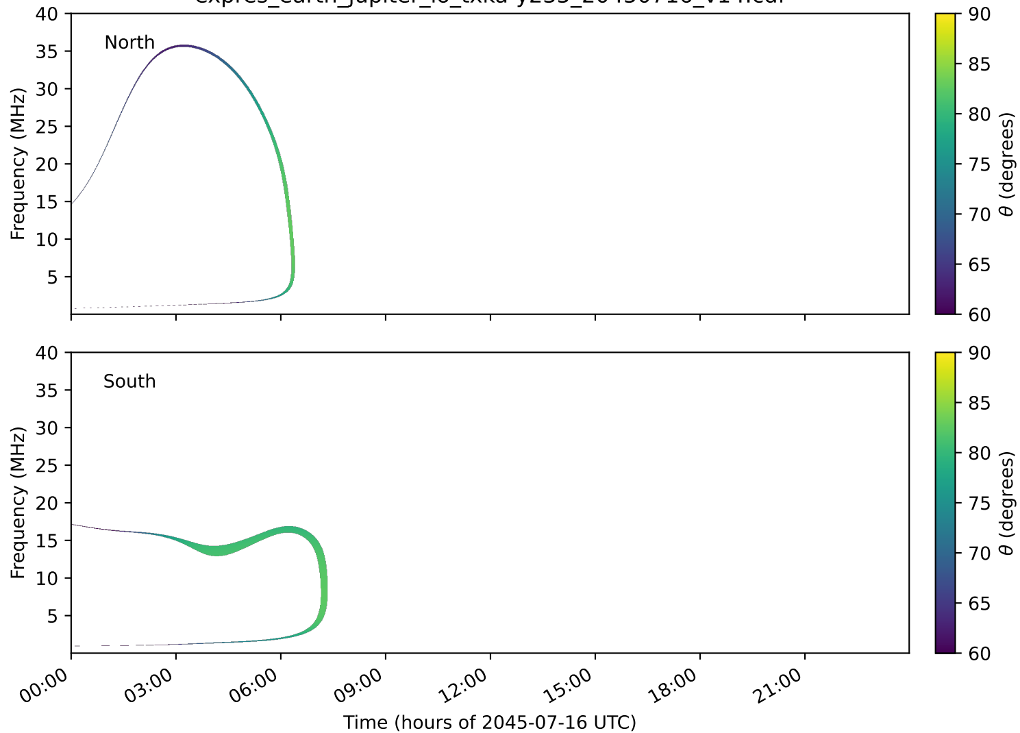
expres_earth_jupiter_io_txka-y235_20450716_v14.cdf
