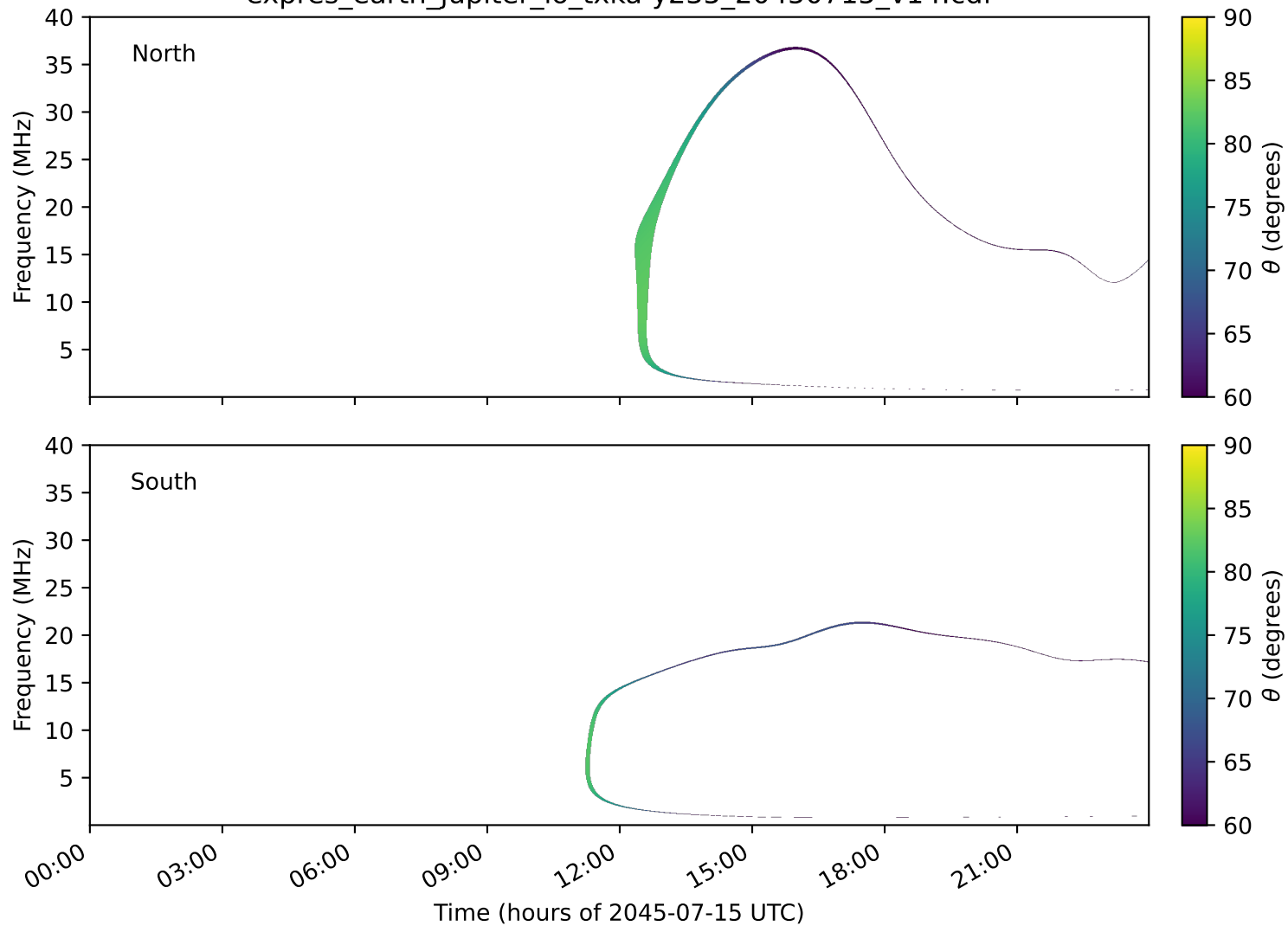
expres_earth_jupiter_io_txka-y235_20450715_v14.cdf
