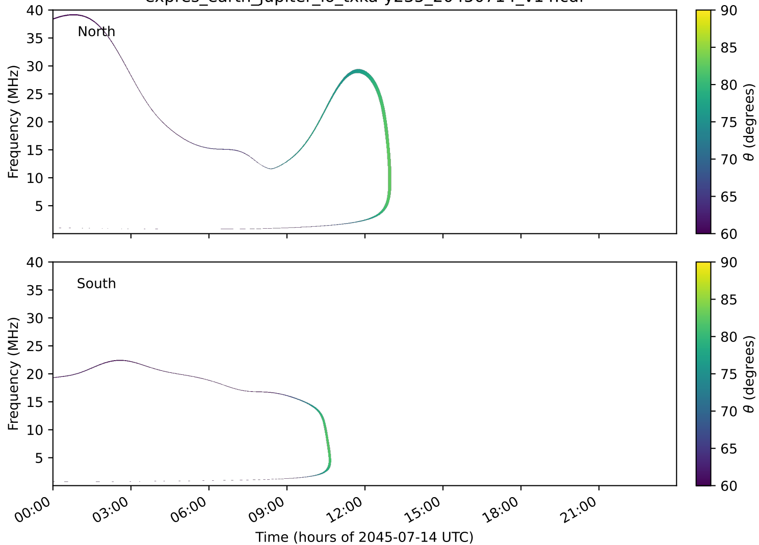
expres_earth_jupiter_io_txka-y235_20450714_v14.cdf
