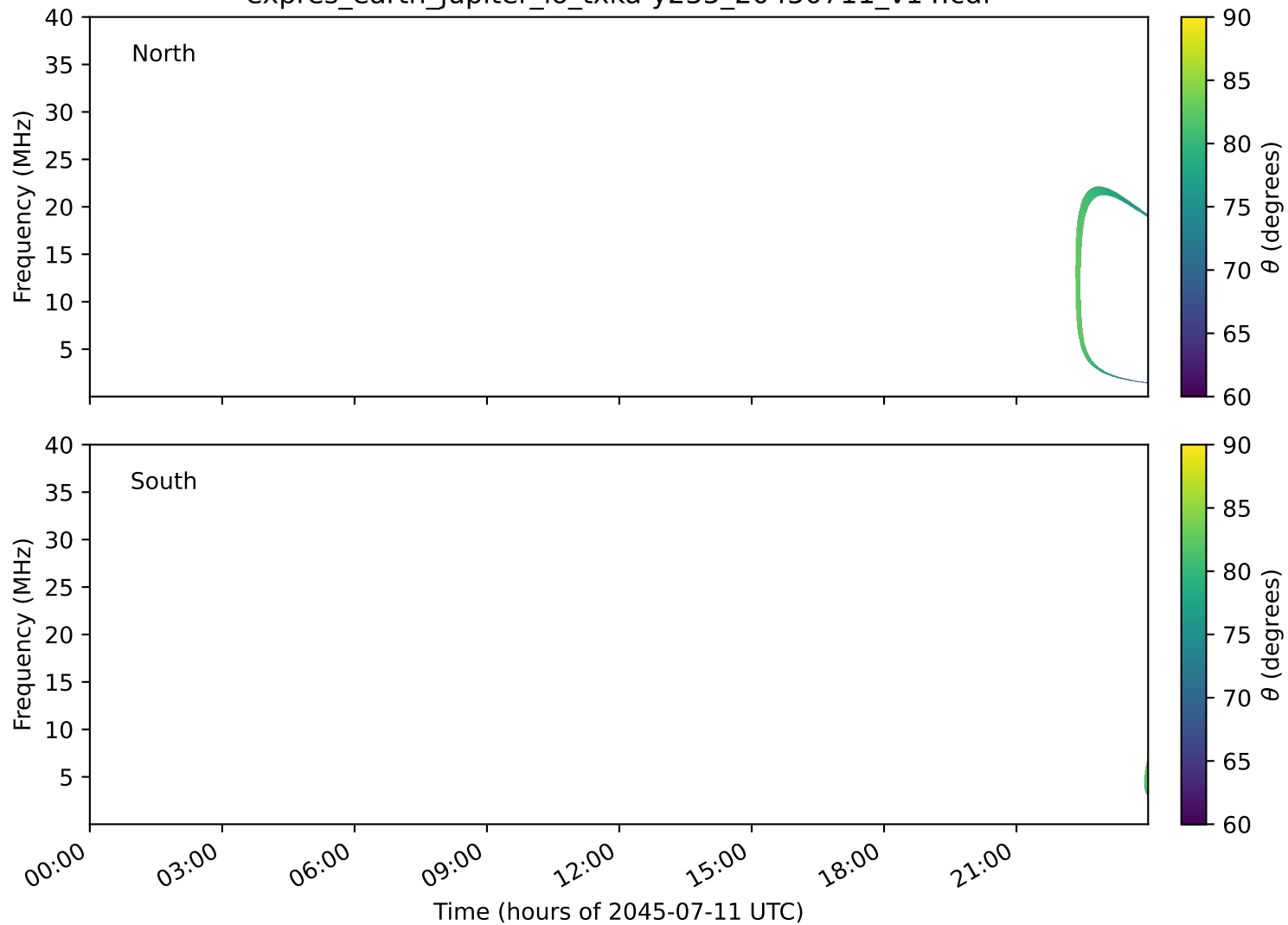
expres_earth_jupiter_io_txka-y235_20450711_v14.cdf
