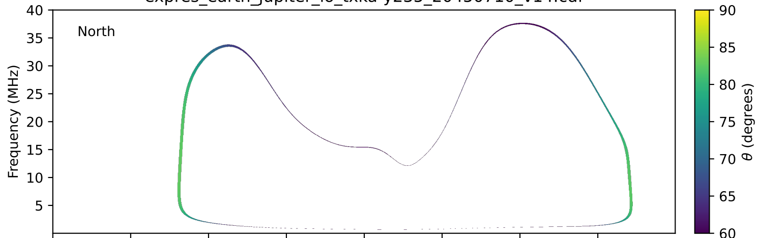
expres_earth_jupiter_io_txka-y235_20450710_v14.cdf
